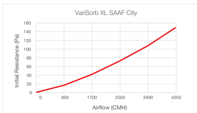
Initial Resistance vs. Airflow
