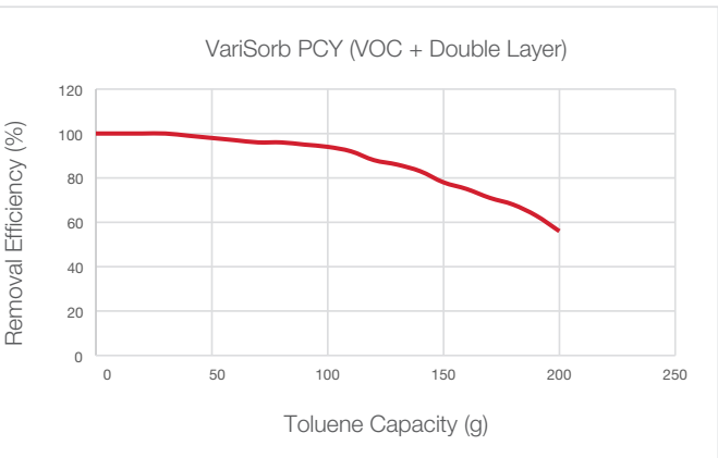
Removal Efficiency Curve
